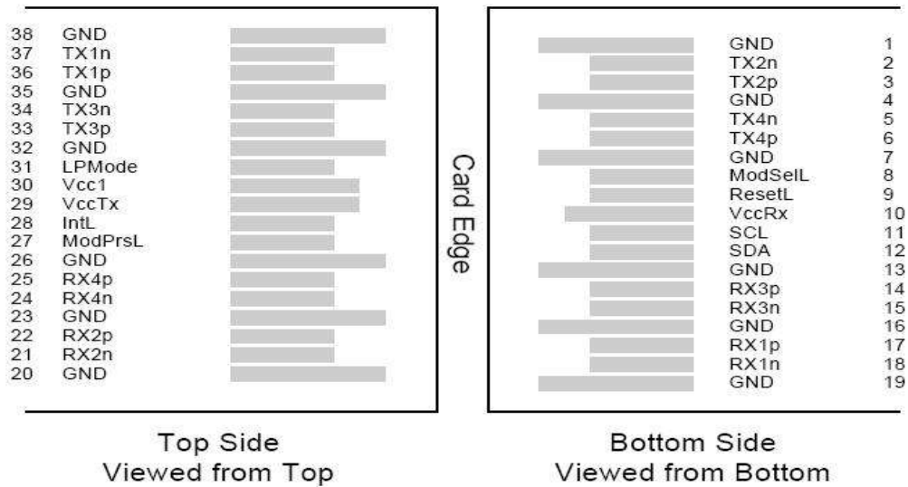
Figure 2: MSA compliant Connector
